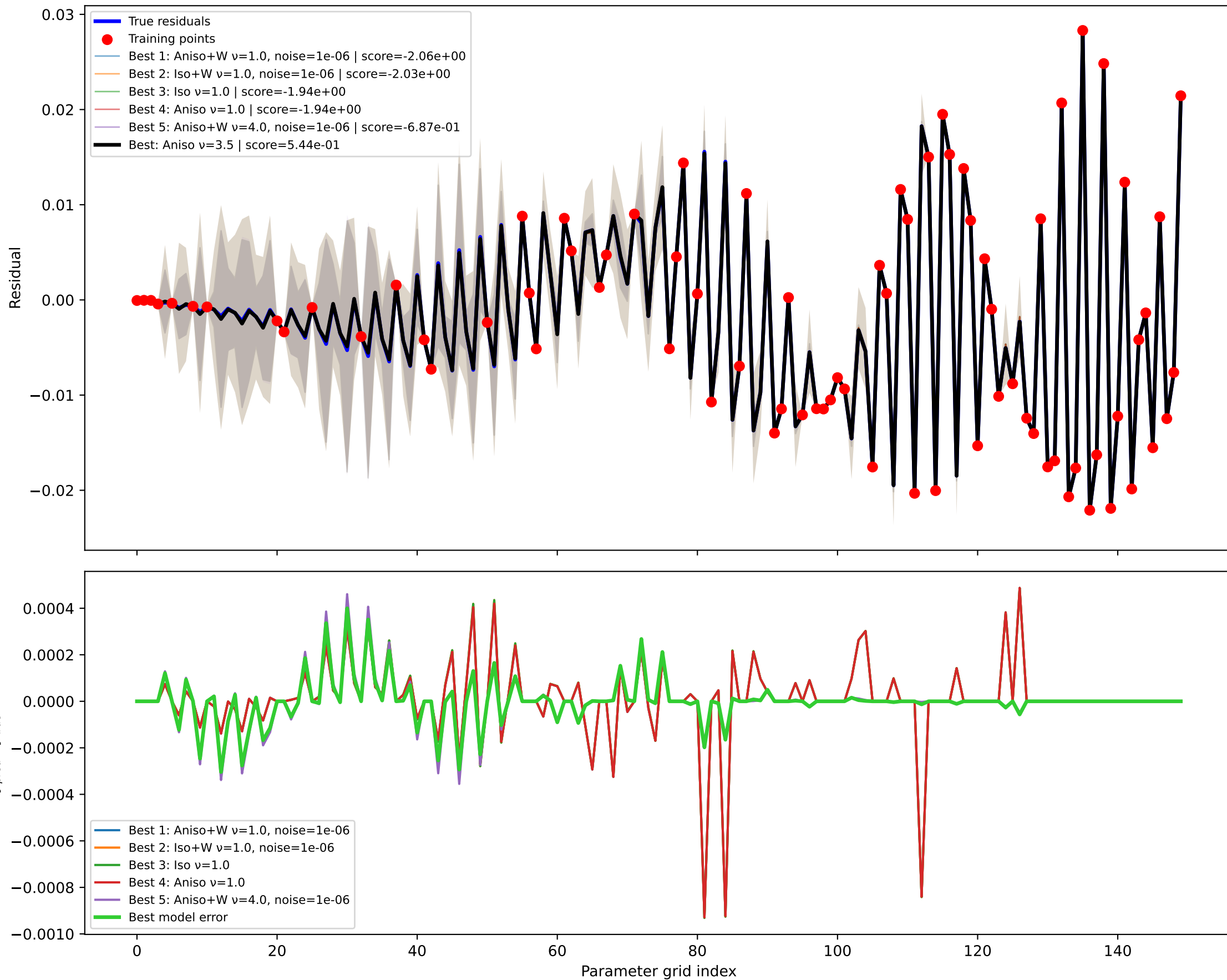
GPR kernel comparison node=14 RMSE=9.537e-05, train RMSE=2.055e-11
